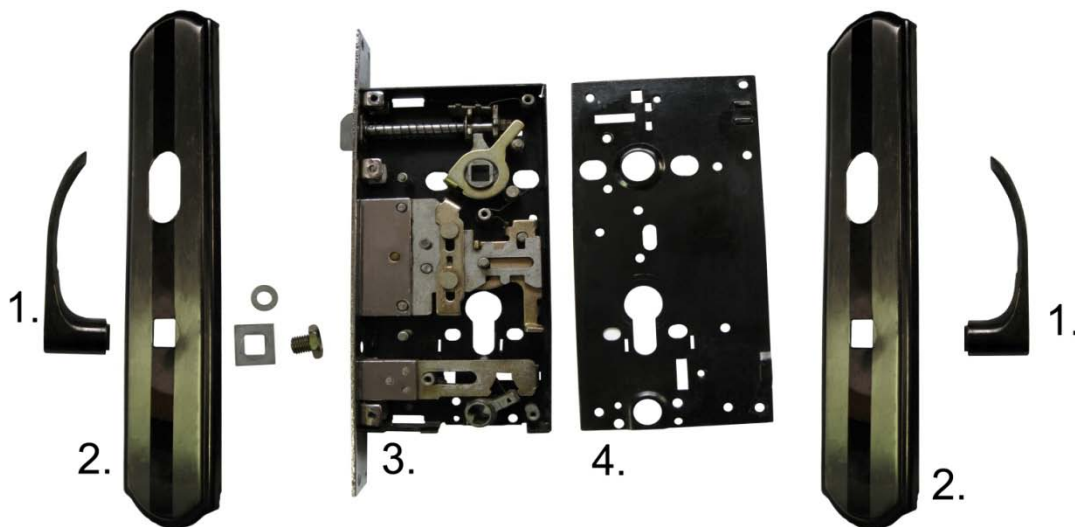
1.lever 2.escutcheon 3.assy, lock unit with faceplate 4.cover
